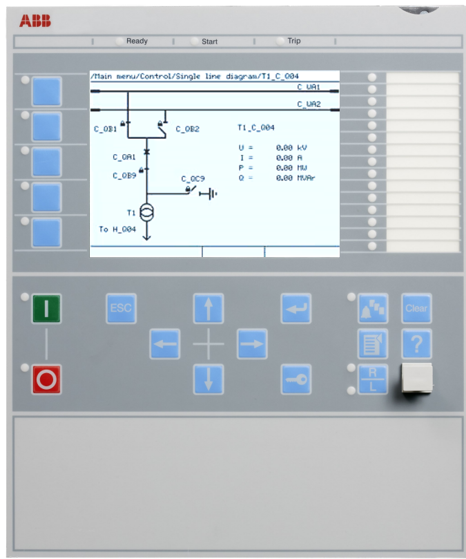
Figure 12. Local human-machine interface
