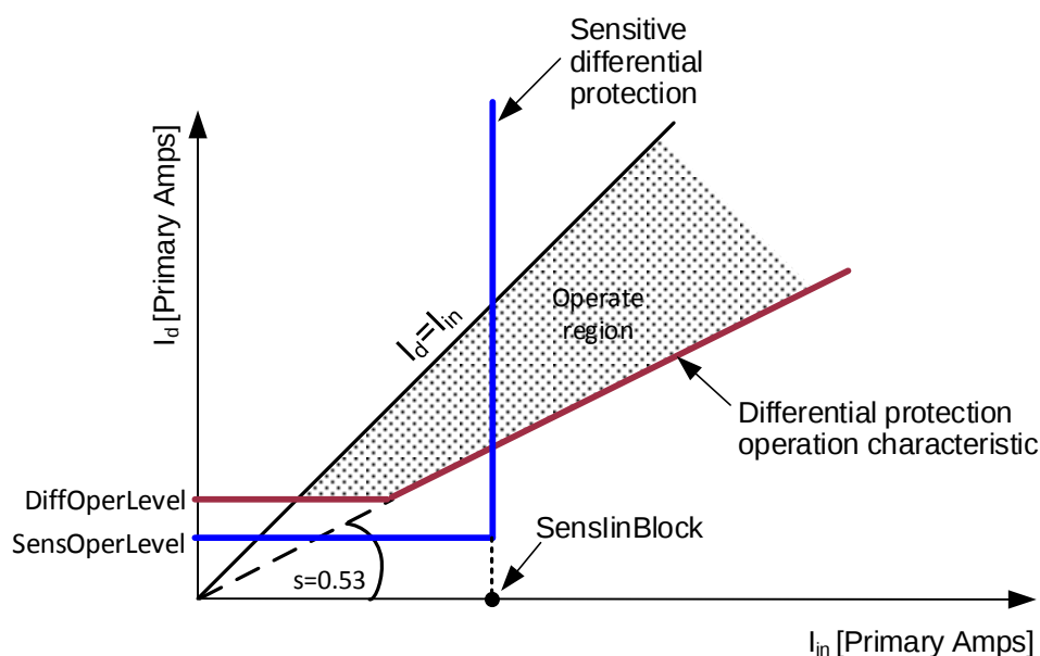
Figure 1. IED operating characteristic
