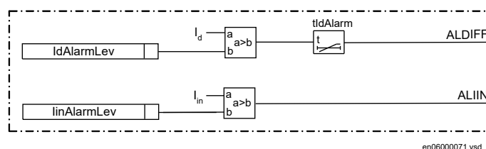
Figure 11. Simplified logic for Zone supervision features
