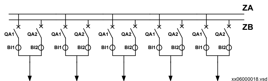
Figure 9. Example of double bus-double breaker station
