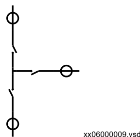
Figure 2. Example of T-connection
