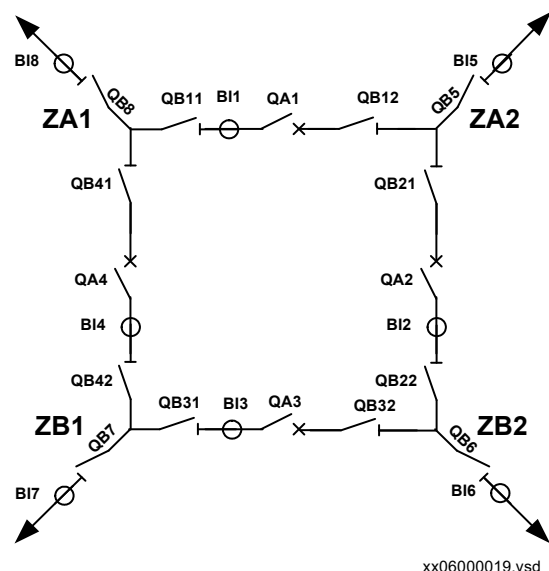
Figure 10. Example of mesh or ring bus station
