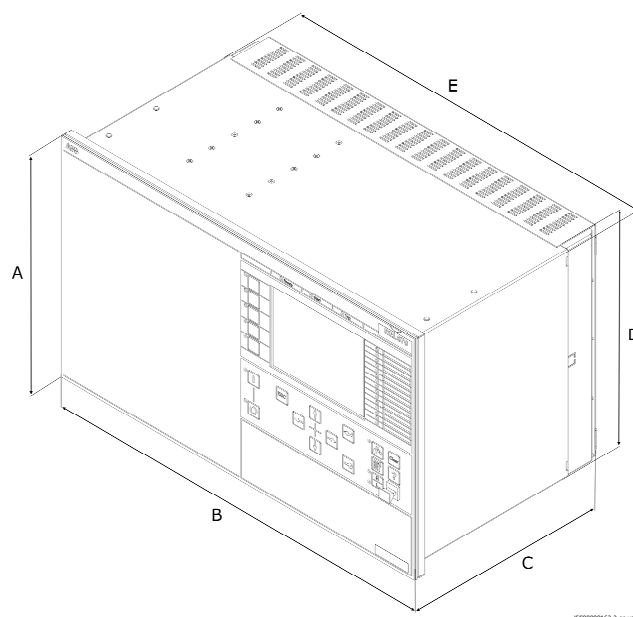
Figure 15. Case with rear cover
