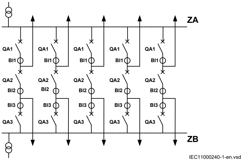
Figure 8. Example of one-and-a-half breaker station
