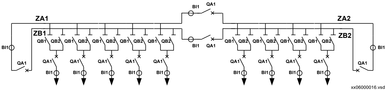
Figure 7. Example of double bus-single breaker station with two bus-section and two bus-coupler breakers (typical GIS station layout)
