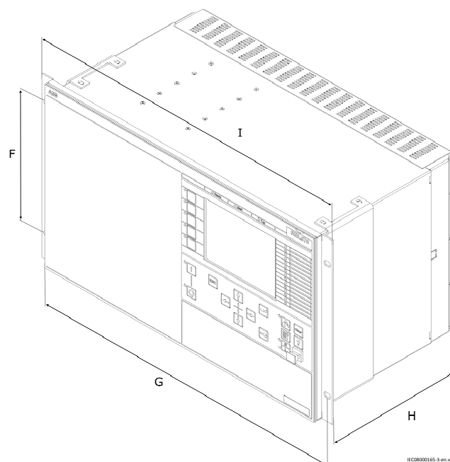
Figure 16. Case with rear cover and 19" rack mounting kit
